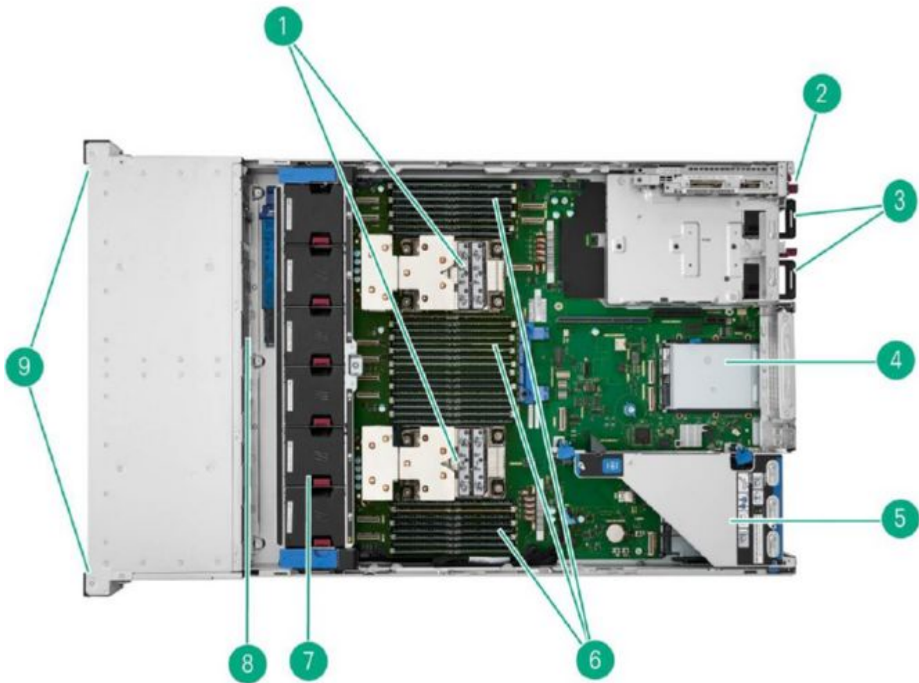
Internal View SFF chassis- Air Cooled
