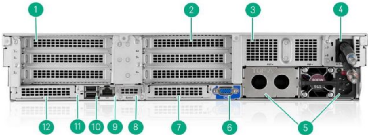
Rear View - DL380 Gen12 Direct Liquid Cooling
